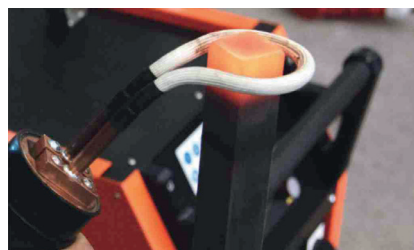
Rods heating
